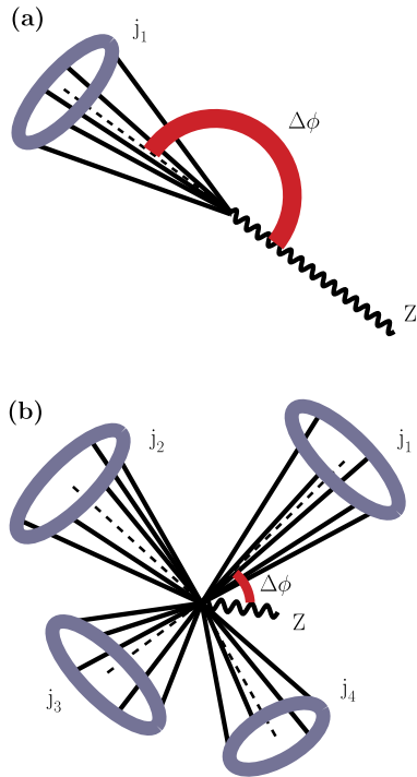
Fig. 1. Topology of Z + jets events: (a) for \ln \tau_T \rightarrow -\infty and \Delta\phi(Z, j_1) \rightarrow \pi ; (b) for \ln \tau_T \rightarrow -1 and \Delta\phi(Z, j_1) \ll \pi .
