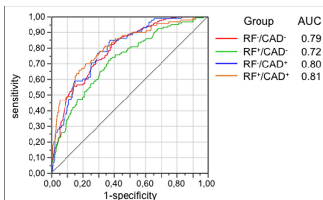
FIGURE 3 | Ability of the 12 proteins selected from Table 3 to predict groups as tested by the area-under-curve (AUC) of the receiver operating characteristics (ROC) functions. Protein signals were standardized to the median and log-transformed. CAD, coronary artery disease; RF, risk factor.
