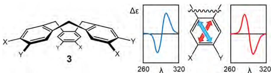
FIGURE 4 Chiral cyclotrimeratrienes studied by Collet and coworkers. A tilt of 1 L b TDM in the direction of red arrow produces a negative couplet, and in the direction blue arrow a positive couplet in the 1 L b region, respectively
