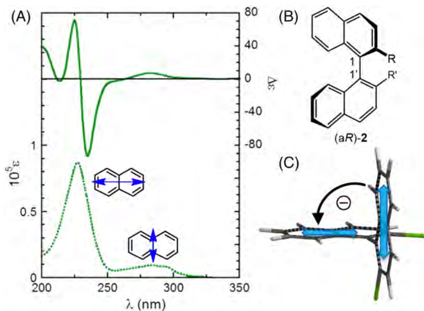
FIGURE 3 Application of the ECM to 1,1'-binaphthyls ( 2 ). (A,B) Diagram and ECD spectrum of (aR)-2,2'-bis(chloromethyl)-1,1'-binaphthalene (R = CH 2 Cl, acetonitrile) showing a negative exciton couplet in the region of the long-axis transition. (C) Chirality defined by the two transition dipoles: A negative chirality (and couplet) is found for (aR) axial chirality
