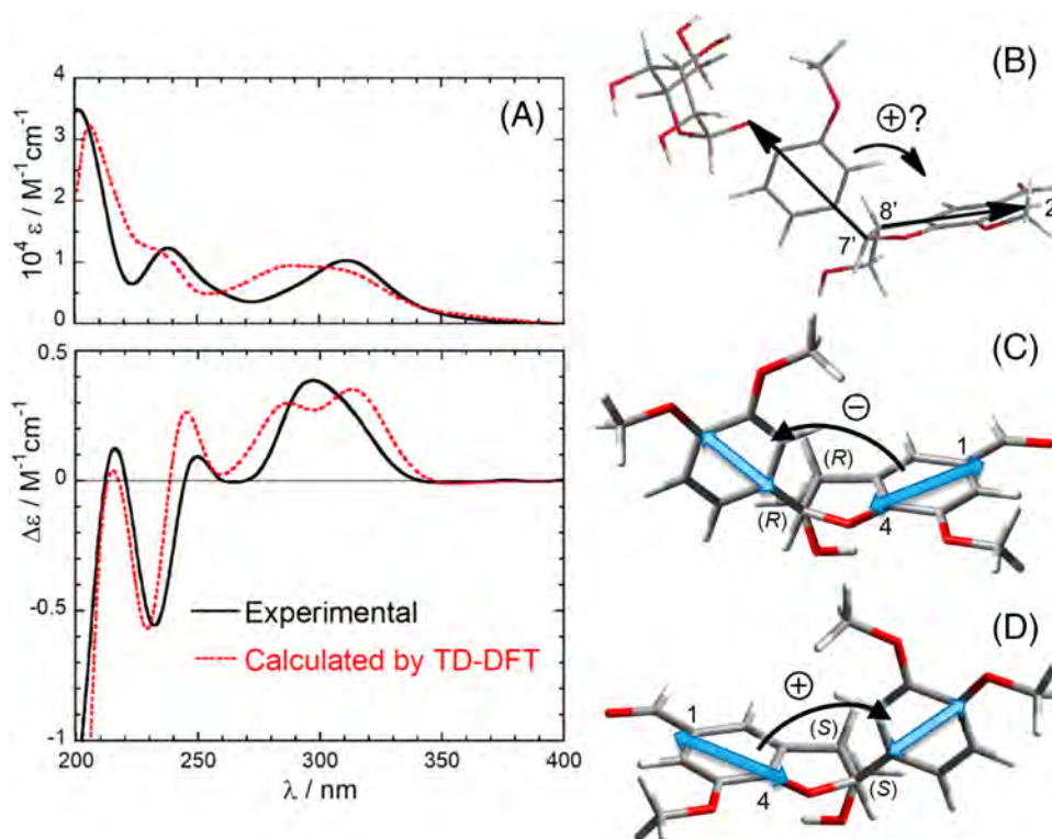
FIGURE 5 Application of the ECM and ECD calculations to ligusticumldehyde A ( 4 ). (A) Experimental UV (top) and ECD (bottom) spectra (methanol) compared with the TD-DFT calculated spectra for model (7'S,8'S)- 4a (this work). (B) Supposed positive helicity defined by the two transition dipoles for 4* . (C) Negative helicity defined by the two transition dipoles shown on the lowest energy conformer of (7'R,8'R)- 4a . The direction of the TDM on the right was established by TD-DFT calculations on 7-methoxy-3-methyl-2,3-dihydrobenzofuran-5-carbaldehyde. (D) Correct positive exciton chirality for the revised configuration (7'S,8'S)- 4a . Experimental spectra and panel (b) adapted from ref. 69 Copyright 2018, with permission from Elsevier. See Supporting Information for calculation details
