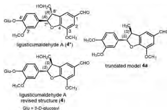
SCHEME 2 Diagram of the original structure of ligusticualdehyde A ( 4* ), its revised structure ( 4 ), and the truncated model used in our analysis ( 4a )
