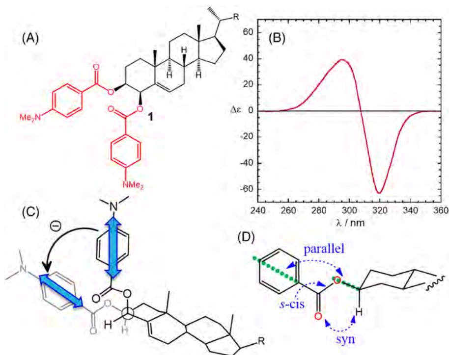
FIGURE 2 Application of the ECM to cholest-5-ene-3 \beta ,4 \beta -diol bis( p -dimethylaminobenzoate) ( 1 ).
