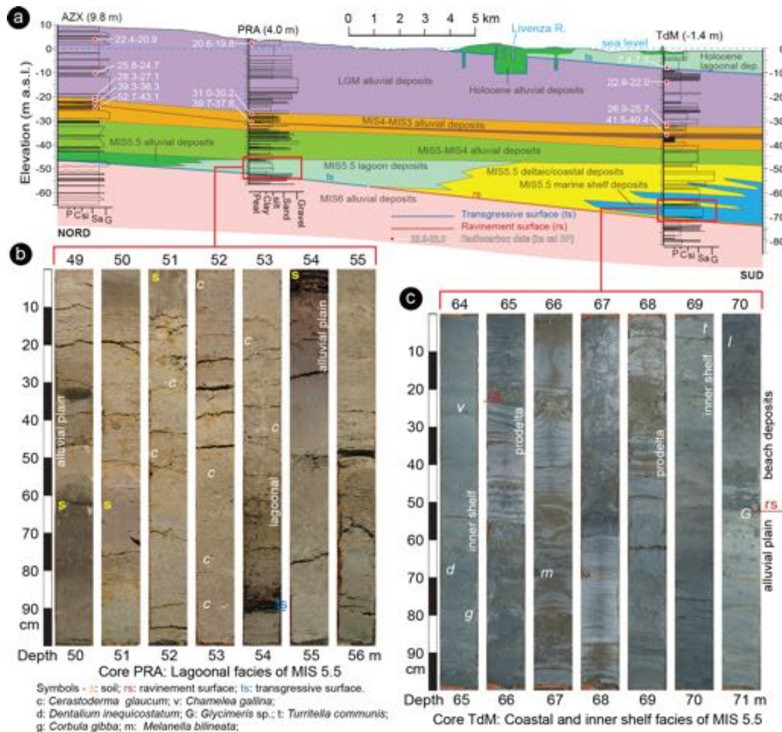
Figure 27. (a) Stratigraphic section of the Venetian Friulian Plain, from the AZX Azzano core (RSL ID 1301, no. 8 in Fig. 28) via the PRA Belfiore core (RSL ID 793, no. 7 in Fig. 28) to the TdM Torre di Mosto core (RSL ID 1295, no. 6 in Fig. 28) (modified from Fontana et al., 2010). The trace of the section is indicated in Fig. 28. (b) Part of core PRA from 49 to 55 m of depth with typical sedimentary facies of a lagoonal environment. (c) Interval of core TdM from 64 to 71 m of depth with typical facies of the basal part of the MIS 5e marine transgression.
