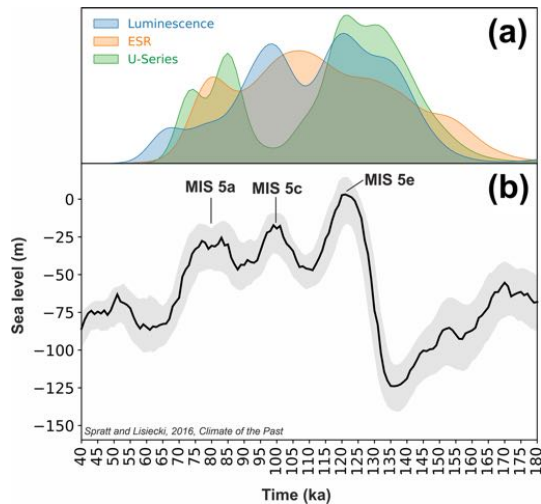
Figure 4. (a) Kernel density estimate plots for luminescence, ESR and U-series samples for which a radiometric age is available in the western Mediterranean database. This plot has been obtained by Monte Carlo sampling ( n = 100\,000 ) the normal distribution of each dated sample in the western Mediterranean database and plotting the resulting age distributions. (b) Late Pleistocene sea level from Spratt and Lisiecki (2016).
