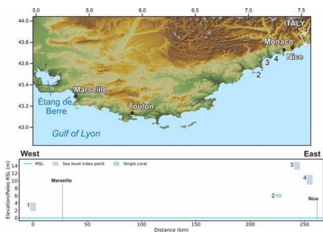
Figure 14. MIS 5 sea-level data for Provence-Côte d'Azur (France). Upper panel: map of sites. The topography has been obtained from the SRTM void-filled DEM (Farr et al., 2007, NASA dataset). Lower panel: distance/elevation graph, from west (left) to east (right). Sites list: 1: Étang de Berre (RSL ID 387); 2: Cap d'Antibes (USeries_1988); 3: Nice Le Bosquet (RSL ID 449); 4: Nice Les Amandier (RSL ID 451).
