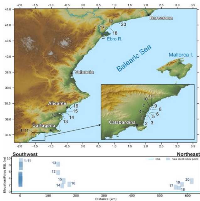
Figure 10. MIS 5 sea-level data for Murcia, the Valencian Community, and Catalonia. Upper panel: map of sites. The topography has been obtained from the SRTM void-filled DEM (Farr et al., 2007, NASA dataset). Lower panel: distance/elevation graph from the southwest (left) to the northeast (right). Sites list: 1: Cope Basin – Point 11 Unit D (RSL ID 750); 2: Cope Basin – Point 10 Unit D (RSL ID 749); 3: Cope Basin – Point 9 Unit D (RSL ID 748); 4: Cope Basin – Point 8 Unit D (RSL ID 747); 5: Cope Basin – Point 7 Unit D (RSL ID 746); 6: Cope Basin – Point 6 Unit D (RSL ID 745); 7: Cope Basin – Point 4 Unit D (RSL ID 743); 8: Cope Basin – Point 5 Unit D (RSL ID 744); 9: Cope Basin – Point 3 Unit D (RSL ID 742); 10: Cope Basin – Point 2 Unit D (RSL ID 741); 11: Cope Basin – Point 1 Unit D (RSL ID 740); 12: La Marina – El Pinet Section B, Terrace T8 (RSL ID 738); 13: La Marina – El Pinet Section A, Terrace T8 (RSL ID 751); 14: south of Torre de Enmedio (RSL ID 4079); 15: Calabasi (RSL ID 4080); 16: Cabo de las Huertas (RSL ID 4081); 17: Morro del Gos (RSL ID 4002); 18: Cala del Torrent del Pi (RSL ID 4084); 19: Cala de Gestell (RSL ID 4083); 20: Cabo de Salou Cala Font (RSL ID 4082).
