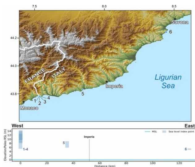
Figure 15. MIS 5 sea-level data for Liguria (Italy). Upper panel: map of sites. The topography has been obtained from the SRTM void-filled DEM (Farr et al., 2007, NASA dataset). Lower panel: distance/elevation graph, from west (left) to east (right). Sites list: 1: Ex Casino (RSL ID 240); 2: Barma Grande (RSL ID 233); 3: Bausu da Ture (RSL ID 239); 4: Grotta del Principe (RSL ID 237); 5: Madonna dell'Arma (RSL ID 242); 6: Grotta Marina di Bergeggi (RSL ID 246).
