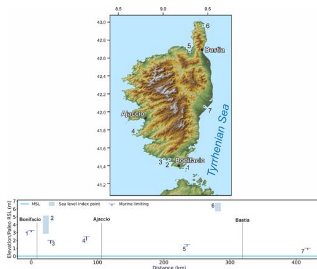
Figure 29. MIS 5 sea-level data for Corsica (France). Upper panel: map of sites. The topography has been obtained from the SRTM void-filled DEM (Farr et al., 2007, NASA dataset). Lower panel: distance/elevation graph, clockwise around the island starting from the southernmost point. Sites list: 1: Piantarella (RSL ID 277); 2: Figari (RSL ID 321); 3: Arbitru (RSL ID 323); 4: Ajaccio Gulf Capo Moru (RSL ID 303); 5: St Florent (RSL ID 299); 6: Macinaccio Tamarone (RSL ID 931); 7: Urbino (RSL ID 322).
