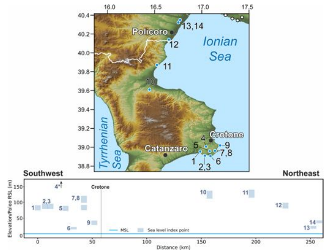
Figure 23. MIS 5 sea-level data for the Ionian side of Calabria and Basilicata (Italy). Upper panel: map of sites. Red dots are sites in the region of interest, and white dots are other sites within the western Mediterranean compilation. The topography has been obtained from the SRTM void-filled DEM (Farr et al., 2007, NASA dataset). Lower panel: distance/elevation graph, from southwest (left) to northeast (right). Sites list: 1: San Leonardo di Cutro (RSL ID 563); 2: Campolongo (RSL ID 4068); 3: Le Castella (RSL ID 4069); 4: Manca della Mozza (RSL ID 566, out of bounds at 240 m a.s.l., dated to Marine Isotope Stage 7); 5: Isola di Capo Rizzuto (RSL ID 565); 6: Capo Rizzuto (RSL ID 564); 7: Crotona (II) (RSL ID 3428); 8: Crotona (RSL ID 1379); 9: Capo Colonna Terrace (RSL ID 3634); 10: Vaccarizzo (RSL ID 442); 11: Trebisacce (RSL ID 324); 12: Piano San Nicola (RSL ID 416); 13: Metaponto (RSL ID 4060); 14: Metaponto (II) (RSL ID 4061).
