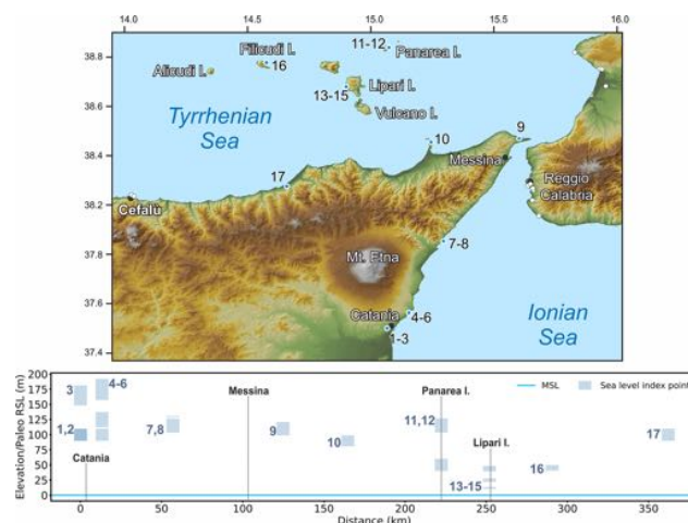
Figure 34. MIS5 sea-level data for Sicily, Sector 4 (Italy). Upper panel: map of sites. Red dots are sites in the region of interest, and white dots are other sites within the western Mediterranean compilation. The topography has been obtained from the SRTM void-filled DEM (Farr et al., 2007, NASA dataset). Lower panel: distance/elevation graph, counterclockwise from Catania to Cefalù. Sites list: 1: Catania (RSL ID 849); 2: Catania (II) (RSL ID 850); 3: Catania (III) (RSL ID 851); 4: Aci Trezza (RSL ID 846); 5: Aci Trezza (II) (RSL ID 847); 6: Aci Trezza (III) (RSL ID 848); 7: Taormina (II) (RSL ID 3626); 8: Taormina (RSL ID 903); 9: Capo Peloro (RSL ID 902); 10: Milazzo (RSL ID 921); 11: Panarea (RSL ID 917); 12: Panarea (II) (RSL ID 918); 13: Lipari (I) (RSL ID 909); 14: Lipari (II) (RSL ID 910); 15: Lipari (III) (RSL ID 911); 16: Filicudi (RSL ID 914); 17: Sant'Agata di Militello (RSL ID 924).
