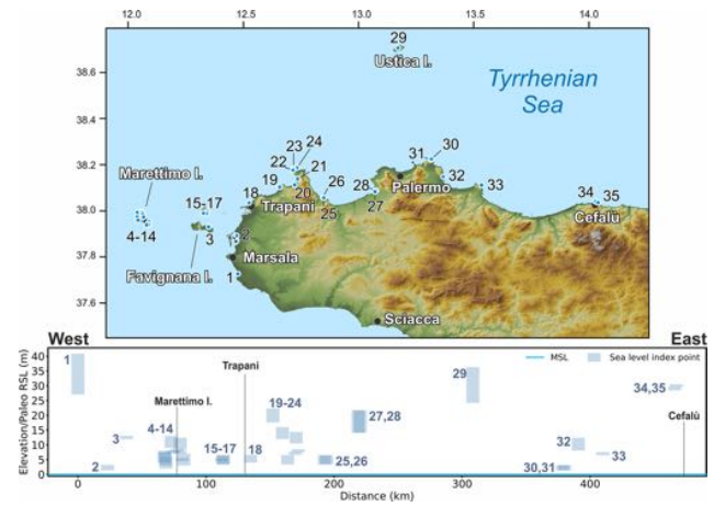
Figure 33. MIS 5 sea-level data for Sicily, Sector 1 (Italy). Upper panel: map of sites. Red dots are sites in the region of interest, and white dots are other sites within the western Mediterranean compilation. The topography has been obtained from the SRTM void-filled DEM (Farr et al., 2007, NASA dataset). Lower panel: distance/elevation graph, from west (left) to east (right). Sites list: 1: Marsala-Mazzaro del Vallo Torre Scibilia (RSL ID 899); 2: Trapani Birgi (RSL ID 919); 3: Favignana Egadi archipelago (RSL ID 855); 4: Facciazzo Marettimo Island (RSL ID 841); 5: Cala Marino Marettimo Island (RSL ID 836); 6: Cala Marino (II) Marettimo Island (RSL ID 840); 7: Cala Conca Marettimo Island (RSL ID 842); 8: Cala Nera Marettimo Island (RSL ID 843); 9: P. Pegna Marettimo Island (RSL ID 837); 10: P.ta Due Frati Marettimo Island (RSL ID 833); 11: Scalo Maestro Marettimo Island (RSL ID 834); 12: Tuono Marettimo Island (RSL ID 838); 13: Sco. Camello Marettimo Island (RSL ID 835); 14: Passo del Bue Marettimo Island (RSL ID 839); 15: Pietre Varate Levanzo Island (Egadi archipelago) (RSL ID 854); 16: Cala Dogana Levanzo Island (Egadi archipelago) (RSL ID 852); 17: Cala Fredda Levanzo Island (Egadi archipelago) (RSL ID 853); 18: Trapani- Tonnara S. Giuliano (RSL ID 920); 19: Monte Cofano Trapani (RSL ID 894); 20: Castelluzzo San Vito lo Capo (RSL ID 845); 21: Macari (RSL ID 830); 22: Cala Mancino San Vito lo Capo (RSL ID 844); 23: San Vito lo Capo W side (RSL ID 923); 24: San Vito lo Capo NE side (RSL ID 922); 25: Cala Rossa (RSL ID 828); 26: Cala Bianca (RSL ID 829); 27: Torre San Cataldo (RSL ID 827); 28: Nocella (RSL ID 826); 29: Ustica (RSL ID 916); 30: Palermo Capo Gallo (RSL ID 897); 31: Capo Gallo (RSL ID 832); 32: Palermo (RSL ID 896); 33: Capo Zafferano (RSL ID 831); 34: Cefalù (RSL ID 862); 35: Cefalù (II) La Kalura (RSL ID 863).
