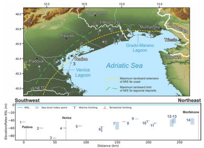
Figure 28. MIS 5 sea-level data for Veneto and Friuli Venezia Giulia (Italy). Upper panel: map of sites. The topography has been obtained from the SRTM void-filled DEM (Farr et al., 2007, NASA dataset). Lower panel: distance/elevation graph, from southwest (left) to northeast (right). The lines depicting the innermost position of the coastline and of the lagoon deposits of MIS 5e are modified after Antonioli et al. (2009). Sites list: 1: Ca' Borille Core (RSL ID 1306); 2: Valle Averte Core CARG 11 (RSL ID 1304); 3: Malamocco Core (RSL ID 1305); 4: VE-1 Core Venezia1 (RSL ID 1303); 5: Portegrandi Core CARG12 (RSL ID 1302); 6: TdM Torre di Mosto Core (RSL ID 1295); 7: PRA Belfiore Core (RSL ID 793); 8: AZX Azzano Core (RSL ID 1301); 9: CNC4 Concordia Sagittaria Core (RSL ID 1289); 10: LUG Lugugnana Core (RSL ID 1294); 11: VV Valle Vecchia Core (RSL ID 1293); 12: Piancada Piancada town (RSL ID 1291); 13: PNC1 Piancada Core (RSL ID 1292); 14: BLG1, Beligna Core (RSL ID 1290). The red line connecting points 6–8 represents the cross section of Fig. 27.
