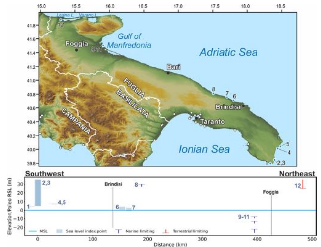
Figure 25. MIS 5 sea-level data for the Adriatic side of Apulia (Italy). Upper panel: map of sites. Red dots are sites in the region of interest, and white dots are other sites within the western Mediterranean compilation. The topography has been obtained from the SRTM void-filled DEM (Farr et al., 2007, NASA dataset). Lower panel: distance/elevation graph, from southwest (left) to northeast (right). Sites list: 1: Grotta del Diavolo (RSL ID 3635); 2: Marina di Novaglie Site (RSL ID 1324); 3: Marina di Novaglie Northern Site (RSL ID 1323); 4: Grotta Romanelli (RSL ID 1319); 5: Grotta delle Striare (RSL ID 1320); 6: Torre Mattarelle - Torre Guaceto (RSL ID 1321); 7: Torre Santa Sabina (RSL ID 1322); 8: Villanova-Monopoli (RSL ID 1318); 9: MM4 borehole Unit 13 (RSL ID 452); 10: MM4 borehole Unit 11 (RSL ID 453); 11: MM4 borehole Unit 10 (RSL ID 454); 12: Fortore River (RSL ID 1317).
