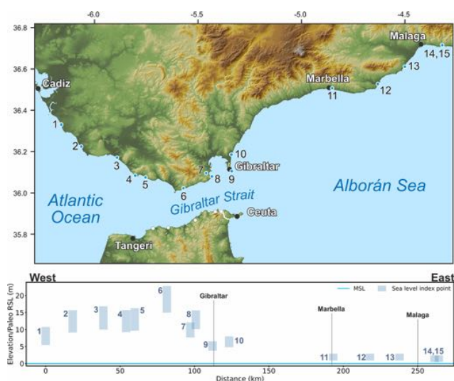
Figure 9. MIS 5 sea-level data for Andalusia (Spain). Upper panel: map of sites. Red dots are sites in the region of interest, and white dots are other sites within the western Mediterranean compilation. The topography has been obtained from the Shuttle Radar Topography Mission (SRTM) void-filled digital elevation model (DEM) (Farr et al., 2007, NASA dataset). Lower panel: distance/elevation graph from west (left) to east (right). Sites list: 1: Torre del Puerco (RSL ID 765); 2: Conil-Trafalgar (RSL ID 764); 3: Zahara (RSL ID 763); 4: Cabo Gracia (RSL ID 762); 5: Bolonia – Punta Paloma (RSL ID 761); 6: Tarifa (RSL ID 760); 7: Algeciras 1 (RSL ID 758); 8: Algeciras 2 (RSL ID 759); 9: Gibraltar (RSL ID 757); 10: La Linea (RSL ID 756); 11: Marbella (RSL ID 755); 12: Fuengirola (RSL ID 754); 13: Torremolinos (RSL ID 753); 14: El Candado (RSL ID 752); 15: Cerro Juan (RSL ID 4001).
