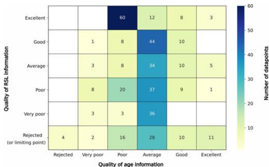
Figure 8. Heatmap summarizing the quality of age and RSL information as estimated within the western Mediterranean database. Numbers in each cell detail the number of sites with the corresponding RSL/age quality ranking. The color of each cell represents the number of sites for each category.
