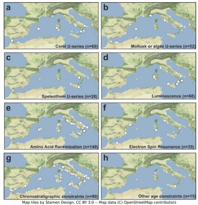
Figure 5. Geographic location of dated samples (or chronostratigraphic attributions), divided by type of analysis. © OpenStreetMap contributors 2020. Distributed under the Open Data Commons Open Database License (ODbL) v1.0.
