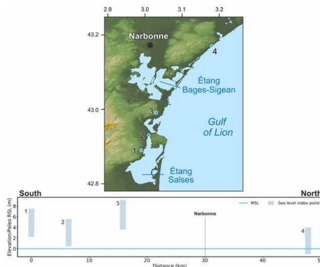
Figure 13. MIS 5 sea-level data for Languedoc-Roussillon (France). Upper panel: map of sites. The topography has been obtained from the SRTM void-filled DEM (Farr et al., 2007, NASA dataset). Lower panel: distance/elevation graph, from south (left) to north (right). Sites list: 1: Leucate Le Malpas (RSL ID 385); 2: Leucate La Franqui (RSL ID 1316); 3: Port la Nouvelle Ramandils (RSL ID 384); 4: Narbonne Saint Pierre (RSL ID 386).
