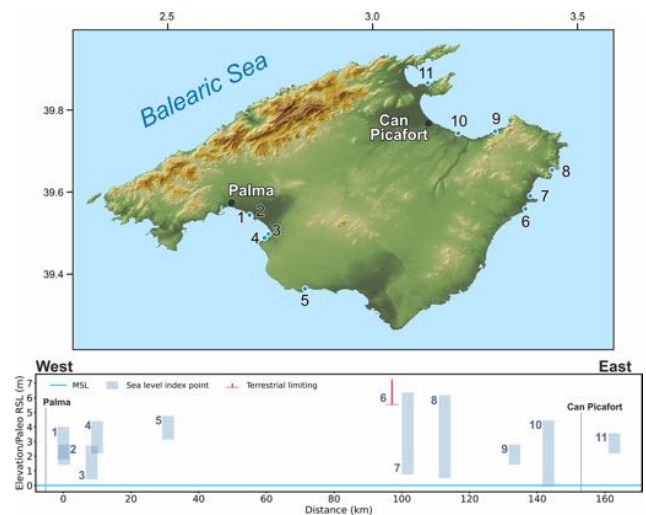
Figure 11. MIS 5 sea-level data for Mallorca (Balearic Islands, Spain). Upper panel: map of sites. The topography has been obtained from the SRTM void-filled DEM (Farr et al., 2007, NASA dataset). Lower panel: distance/elevation graph, counterclockwise from west (left) to east (right). Sites list: 1: Cala Pudent (RSL ID 779); 2: Camp de Tir Unit U4 (RSL ID 357); 3: Cova Baixa (Son Grauet) (RSL ID 780); 4: Cala Blava (RSL ID 781); 5: Cala Pi (RSL ID 782); 6: S'Illot (RSL ID 784); 7: Cala Millor (RSL ID 785); 8: Canyamel (RSL ID 786); 9: Caló des Camps (RSL ID 787); 10: Torrent de Son Real (RSL ID 788); 11: Platja de Sant Joan (RSL ID 789).
