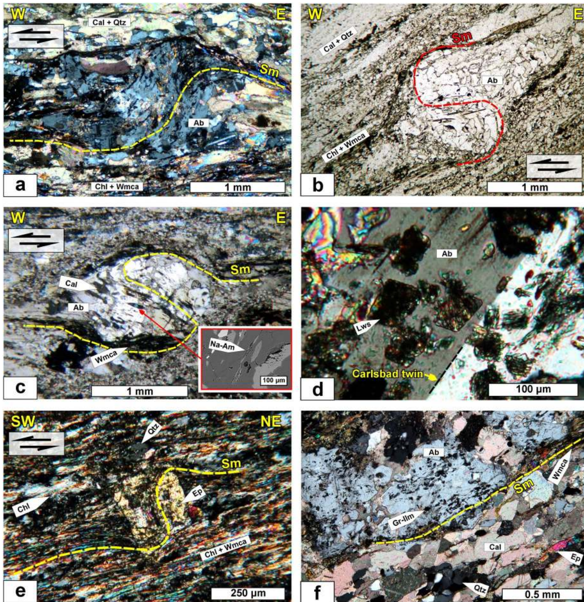
Figure 9. Albite Microstructures: (a and b) Examples of rotated albite porphyroblasts (syn-kinematic; see Passchier and Rudolph [2005]) with sigmoidal internal foliation, defined by oriented inclusions of white mica, chlorite, calcite, and quartz, continuous with the external S_m (a: CPL; b: PPL). (c) Detail of a rotated, syn-kinematic albite porphyroblast containing oriented inclusions of Na-amphibole (CPL). The insert shows a detailed BSE image of the Na-amphibole inclusions, partially resorbed by albite. (d) Detail of misoriented inclusions of lawsonite in albite (CPL). (e) Rotated epidote porphyroblast surrounded by white mica, chlorite, and quartz (CPL). The internal foliation is defined by tiny white mica and graphite inclusions. (f) Example of a post-kinematic albite grain with internal graphite-ilmenite trails continuous with the external foliation (CPL). Notice the lack of strain caps. Mineral abbreviations after Siivola and Schmid (2007).
