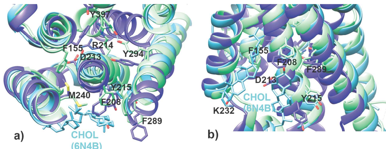
Fig. 7. a) top view and b) front view of S3 cholesterol binding site in superposed 6N4B (agonist and Gi-bound, cyan); 5XRA (agonist bound complex, green) and 5UO9 (antagonist bound, purple). Key residues are visualized.
