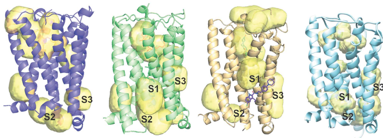
Fig. 6. Summary of receptor cavities predicted by Flap program in 5UO9 structure (Shao et al., 2016) (inactive form), 5XRA 222 (agonist-bound form), 6KQI (Shao et al., 2019) (agonist and NAM bound complex) and 6BN4 26 (agonist and Gi-bound complex).
