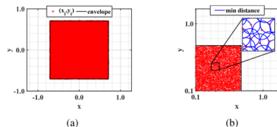
FIGURE 2. Plot (a): Representation of a square domain. Plot (b): Particular for x > 0 and y > 0 .
