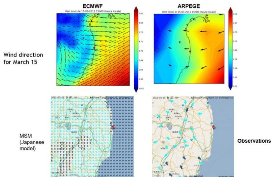
Figure 8. Different observations of wind direction coming from the East and turning over Fukushima to head North-West [34]
