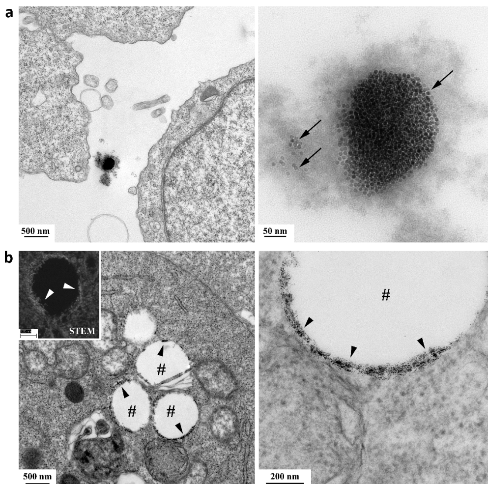
Figure 4. Ultrastructural analysis of Apt-Dend-NP inside MIA-PaCa-2 cells. (a) Metal aggregates found in the extracellular medium; (b) Dendrimer internalization by micropinocytosis mechanism. Arrows = SPIONs aggregate. Arrowheads = Apt-Dend. # = macropinosomes.
