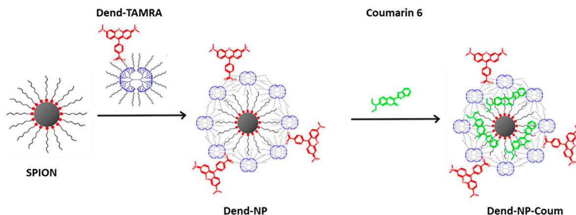
Scheme 1. Synthetic strategy for the assembly of Dend-NP and Dend-NP-Coum.
