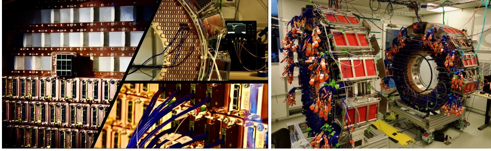
Figure 4: Left: Calorimeter's heart beating. Details of ROU insertion with SiPM facing the crystal and Analog signal at the scope. Right: The calorimeter as of August 2024.
