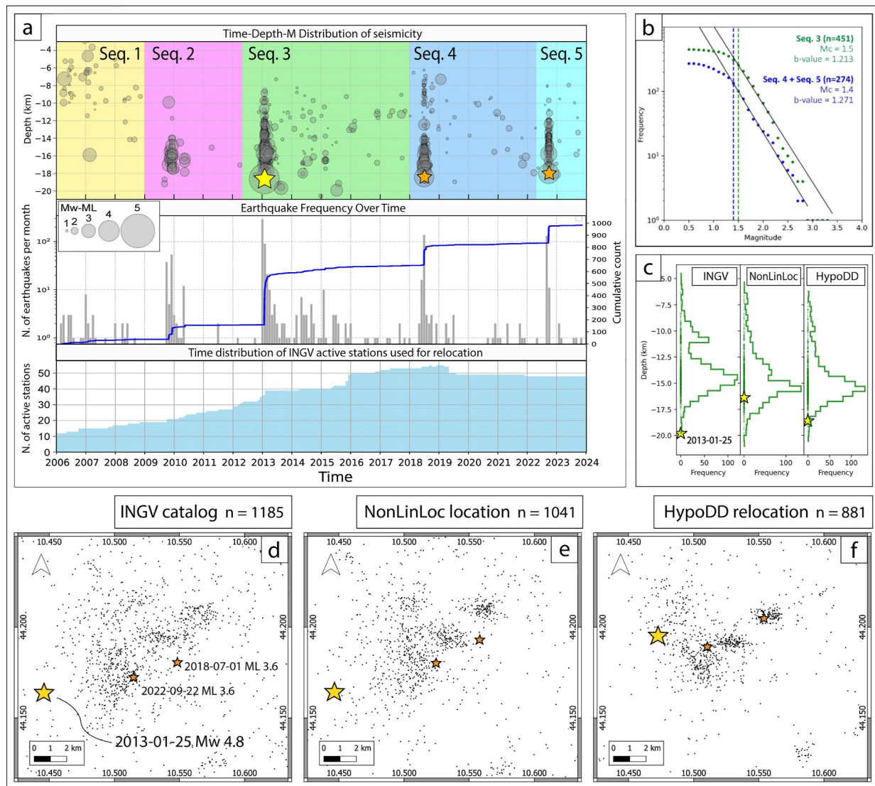
Figure 4. (a) 2006–2024 earthquakes time series, monthly earthquake rate and cumulative active stations through time. Panel (b) m_c and b -value are calculated from original National Institute of Geophysics and Volcanology (INGV) catalog. (c) INGV, NLL, HypoDD catalogs events–depth histograms, with respective depth of the 2013 mainshock. (d)–(f) maps of earthquakes distribution within INGV, NLL and HypoDD catalogs, with stars indicating 2013 (yellow) and 2018–2022 (orange) largest earthquakes.
