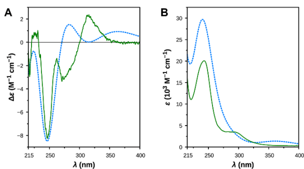
Figure 3. Comparison between the experimental spectra of (–)- 25b (solid lines) and the theoretical spectra of (S)- 25b , as determined by TD DFT calculations (dashed lines). (A) ECD spectra. (B) UV spectra.
