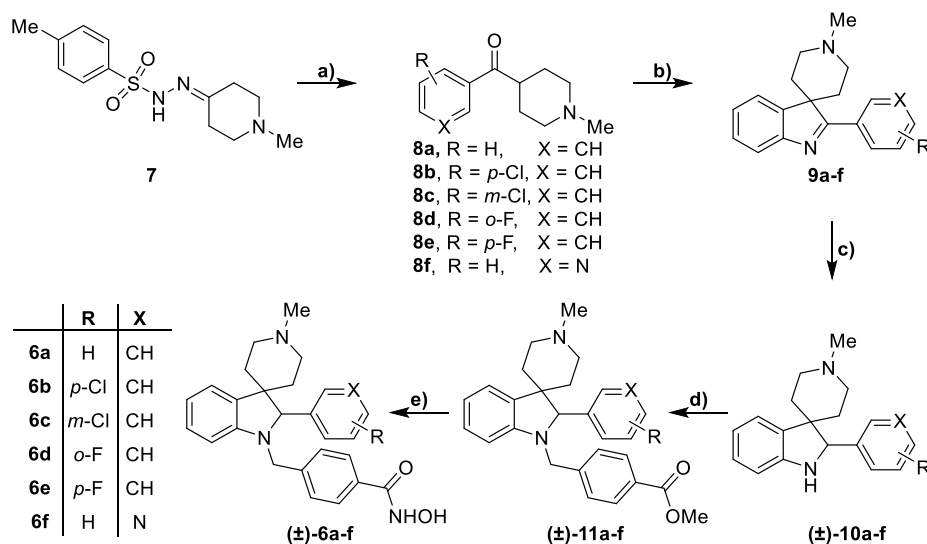
Scheme 1: Synthesis of compounds ( \pm )- 6a-f a
