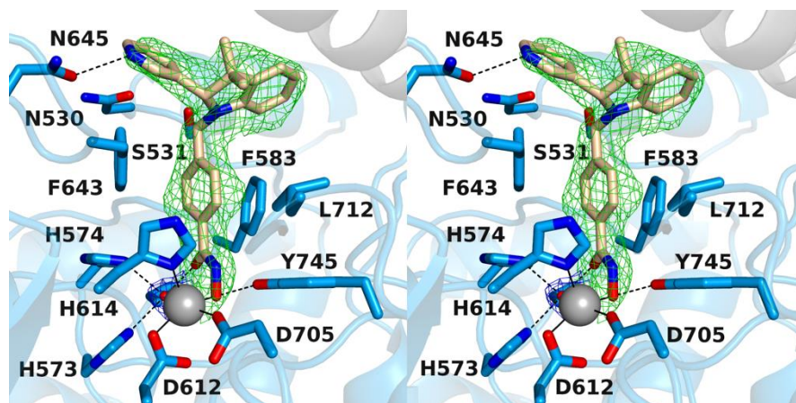
Figure 4. Stereoview of a Polder omit map of the zf HDAC6/( S )- 6h complex (PDB 6V79; contoured at 2.5 \sigma ). The \text{Zn}^{2+} -bound water molecule is contoured at 3.5 \sigma . Atoms are color-coded as follows: C = light blue ( zf HDAC6 monomer A), light gray ( zf HDAC6 monomer B), or wheat (inhibitor), N = blue, O = red, \text{Zn}^{2+} = gray sphere, and \text{Zn}^{2+} -bound water molecule = small red sphere. Metal coordination and hydrogen bond interactions are indicated by solid and dashed black lines, respectively.
