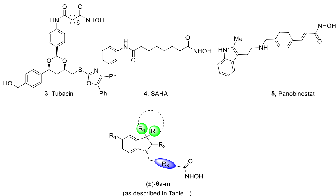
Figure 2. Representative structures of some HDACi as antifibrotic agents and title compounds ( \pm )-6a-m (as described in Table 1).
