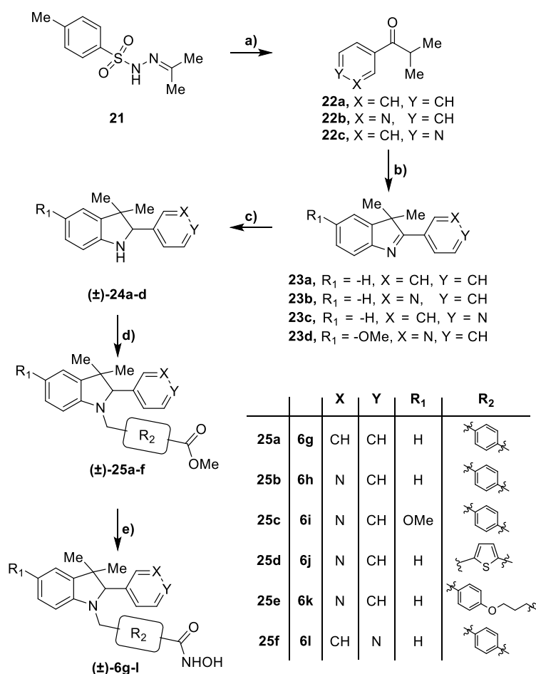
Scheme 3: Synthesis of compounds ( \pm )- 6g-l a
