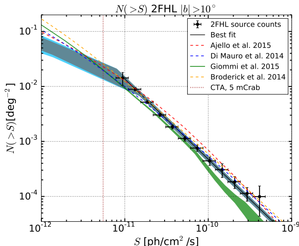
FIG. 4: Cumulative source count distribution N(> S) with the uncertainty bands as in Fig. 3 together with the theoretical predictions from Ref. [12] (blue dashed line), [4] (red dashed line), [13] (green band) and [14] (orange dashed line). The vertical dotted brown line shows the 5 mCrab flux reachable by CTA in 240 hrs of exposure [15].
