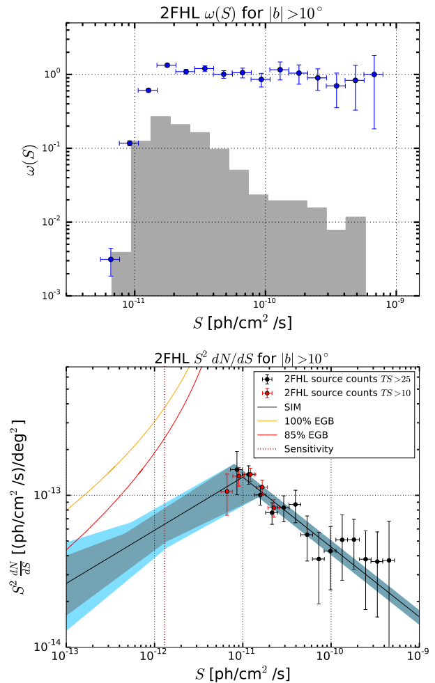
FIG. 3: Top Panel: detection efficiency \omega(S) (blue points) as a function of source flux and normalized distribution of source flux detected in 2FHL (grey shaded histogram). Bottom Panel: intrinsic S^2 dN/dS distribution measured with two different cuts on the source TS : 25 (black points) and 10 (red points, for the lowest four flux bins only). The black solid line shows our best-fit model, while the grey and cyan bands show the 1\sigma and 3\sigma uncertainty bands from the photon fluctuation analysis. The vertical brown dotted line represents the sensitivity of the photon fluctuation analysis. The orange and red curves indicate where 85% and 100% of the EGB intensity above 50 GeV [2]. Taking the 100% curve as an example, any point on that curve, that is joined with a power law to the measured source count distribution at S \approx 10^{-11} \text{ ph cm}^{-2} \text{ s}^{-1} , will give a source count distribution that produces 100% of the EGB.
