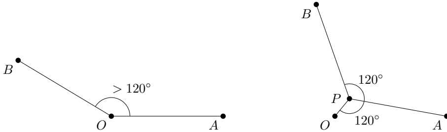
Figure 2. The “ 120^\circ property”. The shortest connected set containing three points A, O, B in two cases.
