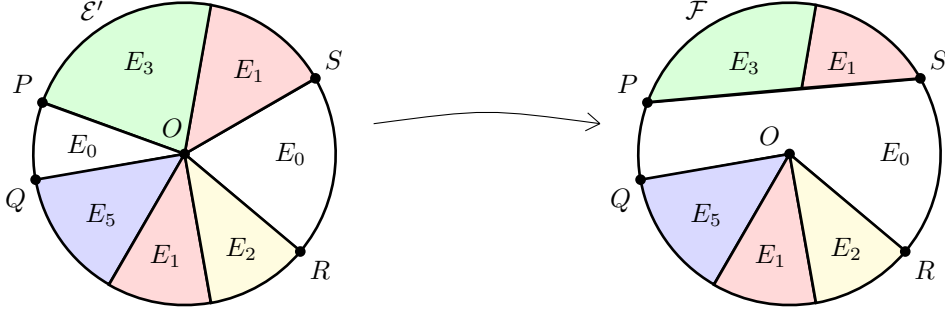
Figure 4. The situation in Step II.
