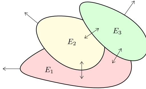
Figure 1. Example of a 3-cluster.
