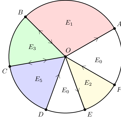
Figure 3. The intersection of a simple cluster with a ball and its perimeter; notice the directions of the arrows.
