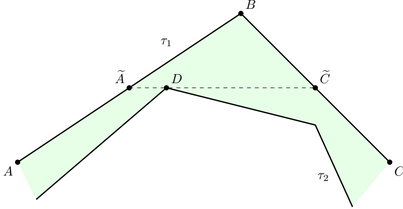
Figure 8. A possible situation in Corollary 2.6.
