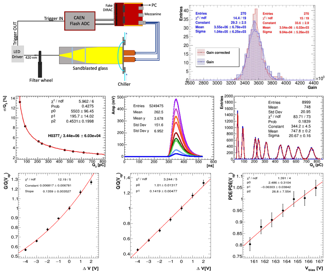
Figure 7. Top-left: test station architecture, including light pulse generator and attenuator. Top-right: distribution of ROU gains for a production batch. Centre: example of SiPM waveforms (middle) and charges (right) for various LED source amplitudes. Centre-left: \sigma_Q / Q fit. Bottom: gain, charge and PDE scans at various overvoltages.
