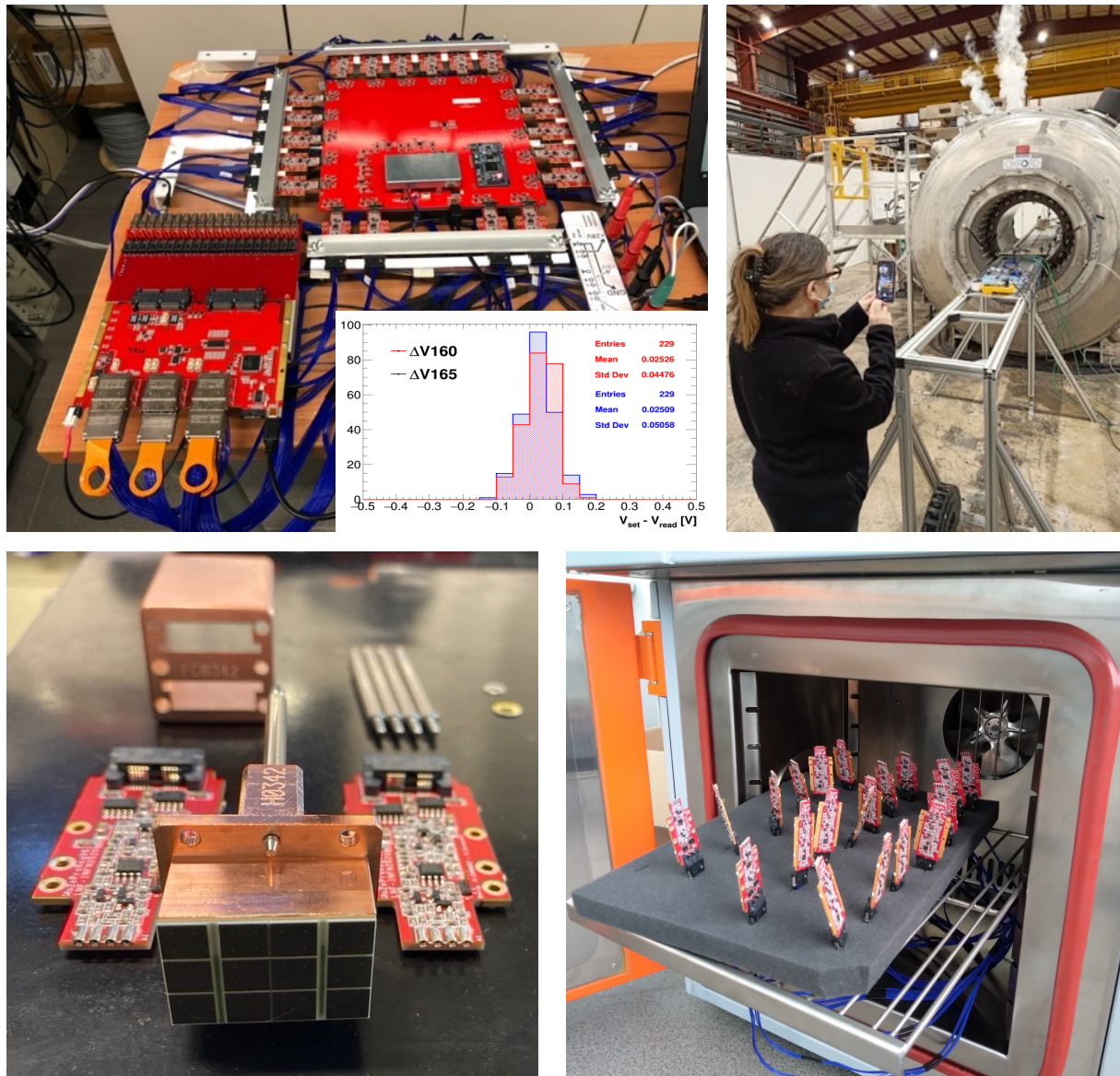
Figure 6. FEE QA bench (top-left), calibration results for HV regulator output are also shown. Test in magnetic fields at Argonne National Laboratory (top-right). ROU before assembly with the FEE boards (bottom-left). FEE burn-in test (bottom-right).
