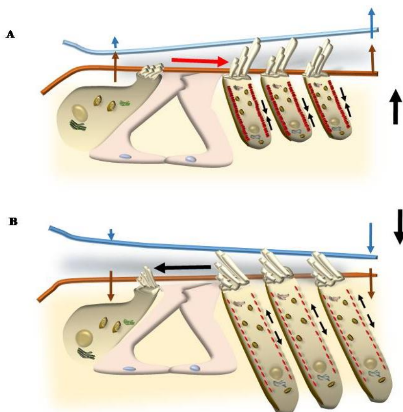
Figure 12. The role of OHC contraction on driving endolymph. During OHC contraction, the gap between TM and RL is increased over OHC (A), which drags more endolymph to move from the smaller volume above IHC towards the greater volume above OHC. This leads an excitatory deflection of IHC stereocilia. Contrary wise, during OHC elongation (B), the space between RL and TM over OHC is compressed and the endolymph flow directs towards IHC, which deflects in the inhibitory way IHC stereocilia. This is the active role of OHC in squeezing the endolymph and enhancing radial shearing. Such a squeezing also occurs in the perilymph of Corti's tunnel which squeezes the pressure orthogonally towards the apex of the cochlea (see text).
