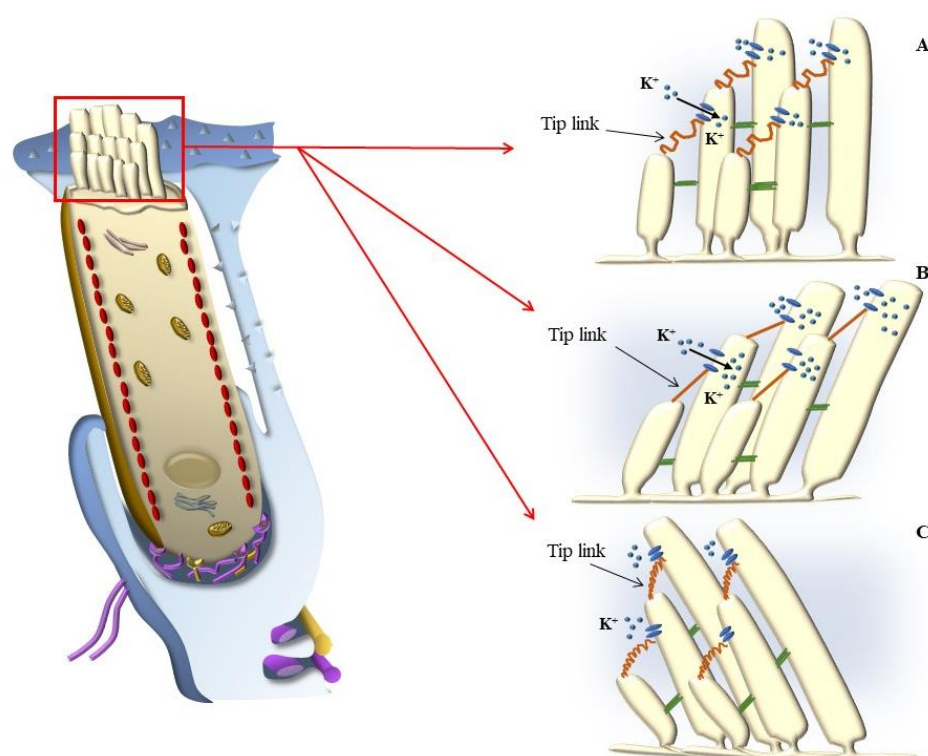
Figure 7. The role of tip links. In resting conditions (A), the position of the SC is orthogonal to the apical membrane of HC. In this condition the tip links, which connect the apex to the lateral membrane of contiguous SC keep a slight tension, which partially keeps protein conformation, within cation channels, which is able produce only partial channel opening. This allows the entry of some cations within HC. During excitation (B), the coordinated movements of SC within the package of each HC, which is granted by lateral links, generate a gradient of tension at the level of the tip links, which connect the apex of a cilium to the lateral membrane of the nearest SC. During excitation the movement is directed towards the longest SC, and the tension of the tip links increases leading to an altered conformation of cation channels, which are more likely to be opened, thus allowing the entry of cations within HC. Contrary wise, when a coordinated movement of SC proceeds from the longest to the shortest SC (C), the tension of the tip links is reduced and the cation channels are no longer mechanically stimulated, which leads to closing the entry of cations.
