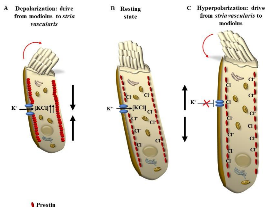
Figure 3. Excitation of OHC reduces, while inhibition increases cell length. When SC deflection occurs in the medio-lateral direction (A, from modiolus to stria vascularis ) a massive cation influx in the OHC takes place which removes anions from the lateral protein named prestin. Such a removal shortens prestin length, which causes cell shortening. In the resting state (B), the entry of cations is moderate and the length of prestin is proportionally increased. In the inhibition phase, when SC deflection occurs in the latero-medial direction (from stria vascularis to modiolus, C) a massive cation efflux from OHC takes place which replaces anions binding to the protein prestin. Such a binding increases prestin length, which causes cell lengthening.
