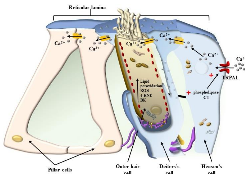
Figure 14. Spreading of excitation from Hensen's cells to external layer of OHC. There is a strict relationship between Hensen's cells and the external layer of OHC. In this way excitation occurring within Hensen's cells may directly propagate through tight junction to OHC.
