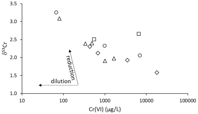
Fig. 9. Cr(VI) vs \delta^{53}\text{Cr} correlation diagram for surface water. The effects of dilution, which leaves the \delta^{53}\text{Cr} unchanged, and Cr(VI) reduction assuming a Rayleigh fractionation law ( \alpha = 0.9958 ; Kitchen et al., 2012) are shown. Symbols are: open circle, September 16, 2022; open square, October 21, 2011; open diamond, November 30, 2022; open triangle, June 15, 2023 surveys.
