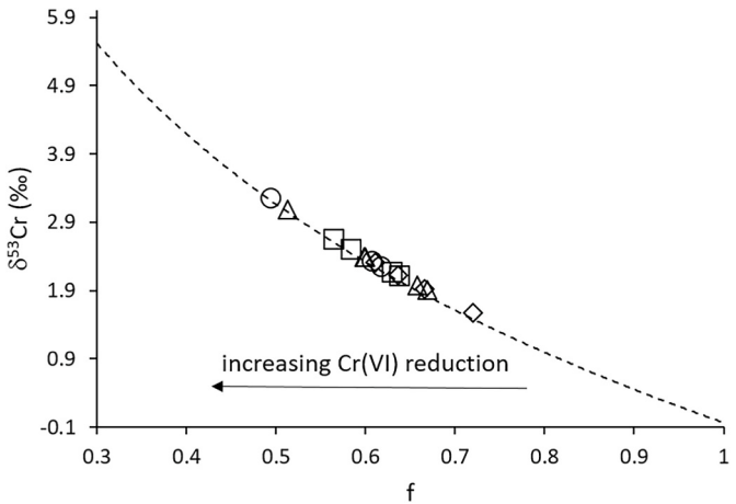
Fig. 10. Fraction of Cr(VI) remaining ( f ) vs \delta^{53}\text{Cr} during progressive reduction, according to a Rayleigh fractionation model ( \alpha = 0.9958 ), for surface waters collected during different surveys and assuming the background Cr isotopic composition of KEU ( \delta^{53}\text{Cr} = -0.031 ). Symbols are: open circle, September 16, 2022 sampling; open square, October 21, 2022; open diamond, November 30, 2022; open triangle, June 15, 2023.
