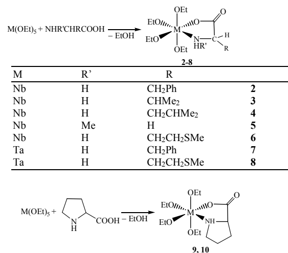
Scheme 1. Reaction of niobium and tantalum pentaethoxides with \alpha -amino acids.
