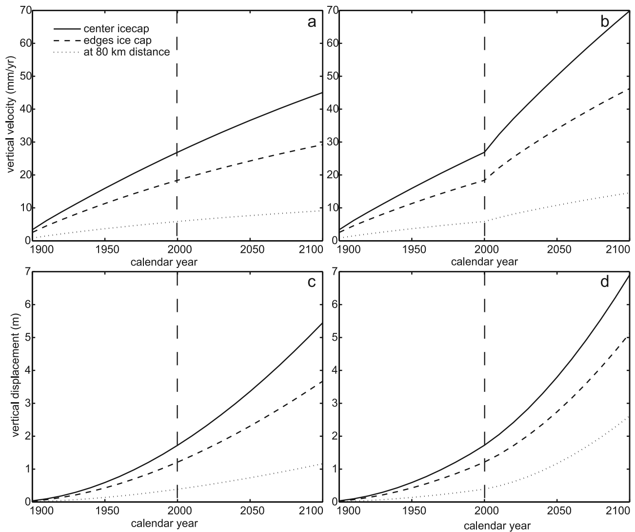
Figure 8. Predicted vertical velocities and displacements at Vatnajökull, assuming an elastic thickness of 10 km and an underlying viscosity of 8 \times 10^{18} Pa s. Lines show the (a) predicted vertical velocities and (c) displacements assuming a thinning rate of 4 \text{ km}^3 until 2100, Figures 8b and 8d show the response if thinning rates were to double in 2000 and remain constant until 2100.
