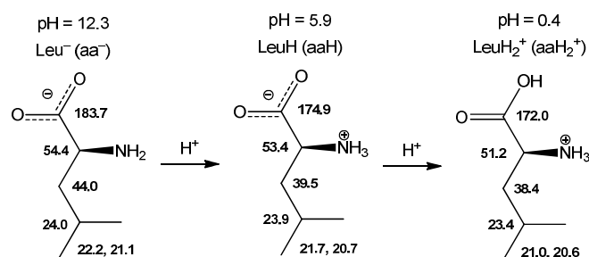
Figure 1 ^{13}\text{C} Chemical shifts at different pH values for L-leucine in \text{D}_2\text{O} . 13(f)
