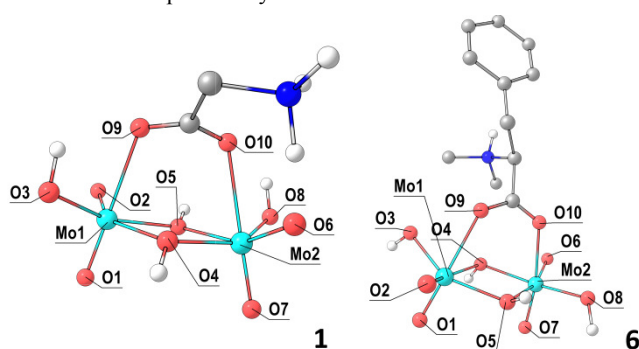
Figure 2 Lowest-energy DFT optimized dinuclear structures of 1 and 6 (gas-phase EDF2 calculations). White = hydrogen, grey = carbon, blue = nitrogen, red = oxygen, light blue = molybdenum. Carbon-bonded hydrogen atoms have been omitted for clarity.
