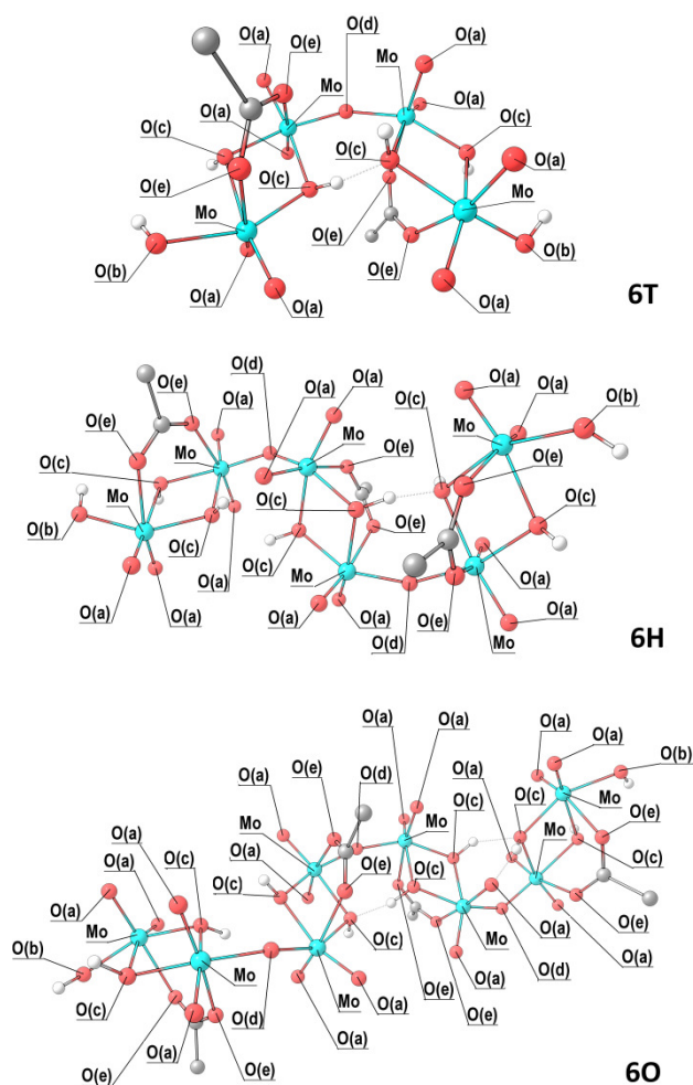
Figure 3 Lowest-energy DFT optimized polynuclear structures of 6 ( 6T , 6H and 6O ) (PBE/Grimme/COSMO, in the presence of water as implicit solvent). White = hydrogen, grey = carbon, blue = nitrogen, red = oxygen, light blue = molybdenum. The substituents on the carboxylate-bonded carbons have been omitted for clarity.
