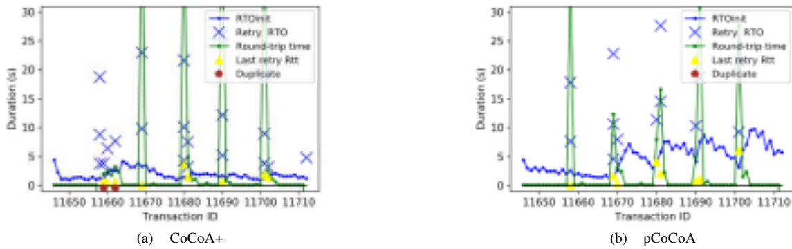
Fig. 21. Weak estimator failing to update RTO_{init} .
