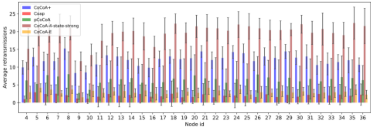
Fig. 16, Node average retransmissions, T = 8s .
