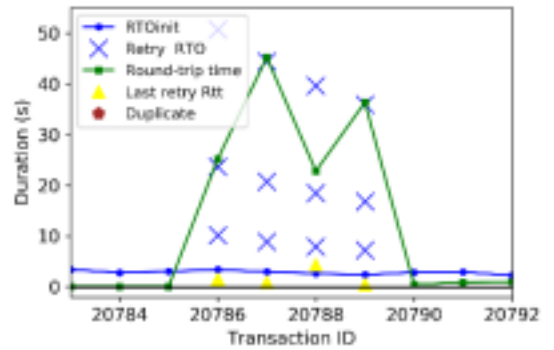
Fig. 11, Weak estimator failing to update RTO_{mit} .
