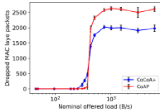
Fig. 3. Overall in-network MAC buffer overflows.
